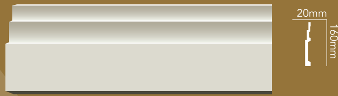
WA-PF160 L:2400mm W:160mm
