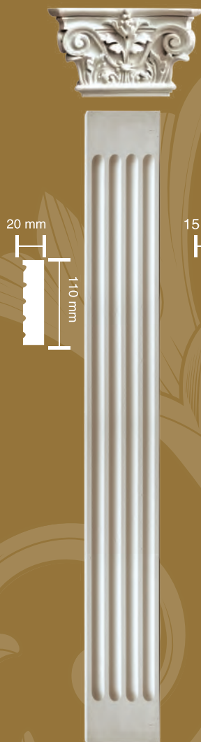
WA-PL010 B 2000x110x20 mm
