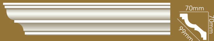
WA-PC139 L:2400mm W:99mm
