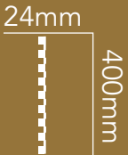
WA-PF170 L:2400mm W:400mm
