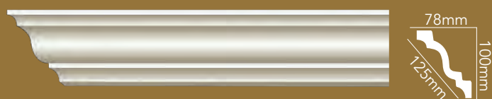
WA-PC068 L:2400mm W:125mm
