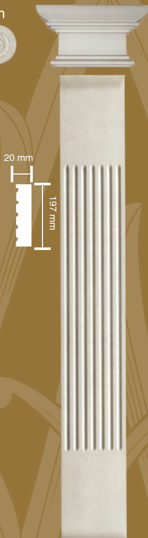
WA-PL012 B 2000x197x20 mm
