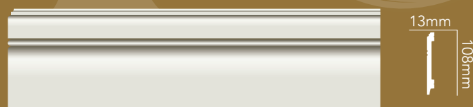
WA-PF163 L:2400mm W:108mm
