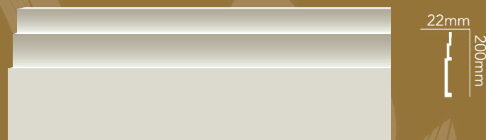
WA-PF161 L:2400mm W:200mm
