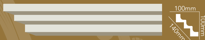
WA-PC082 L:2400mm W:140mm
