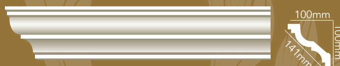
WA-PC141 L:2400mm W:141mm
