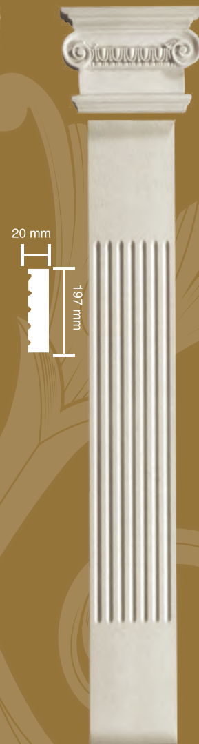
WA-PL002 B 2000x197x20 mm
