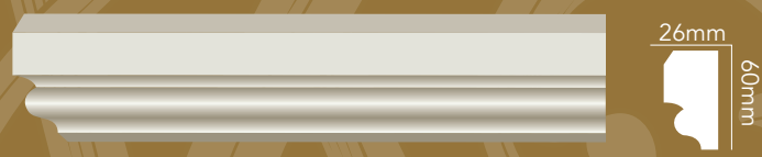
WA-PF078L L:3000mm W:60mm
