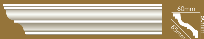
WA-PC138 L:2400mm W:85mm
